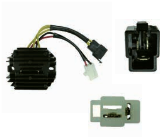
◀ cod. HN1018 Honda Applications 12 Volt Regulator Rectifier Assembly
