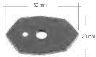
Piastrine frecce Plate for direction indicators PFK2 € 14,50 per 4 pezzi for 4 pieces
